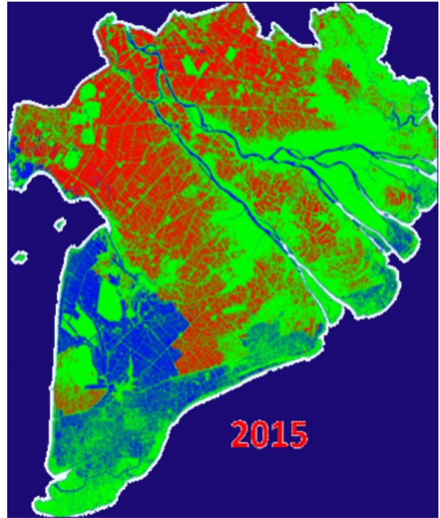
Effect of El Niño on rice crop cultivation, 2015-2016-2017 in the Mekong Delta
