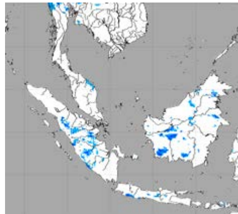
Satellite Detected Region of Extreme Heavy Rainfall based upon percentiles from past 18-yr data
